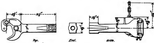
Figs. 3974-3976. Climax Coupler. National Malleable Castings Co.
